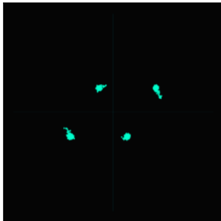
4-HQAM
