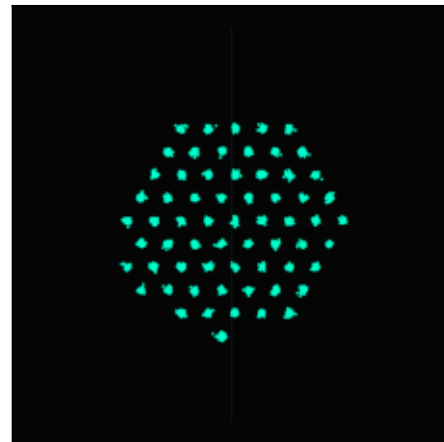
64-HQAM
